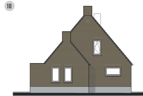
Linkergevel Tweekappers
